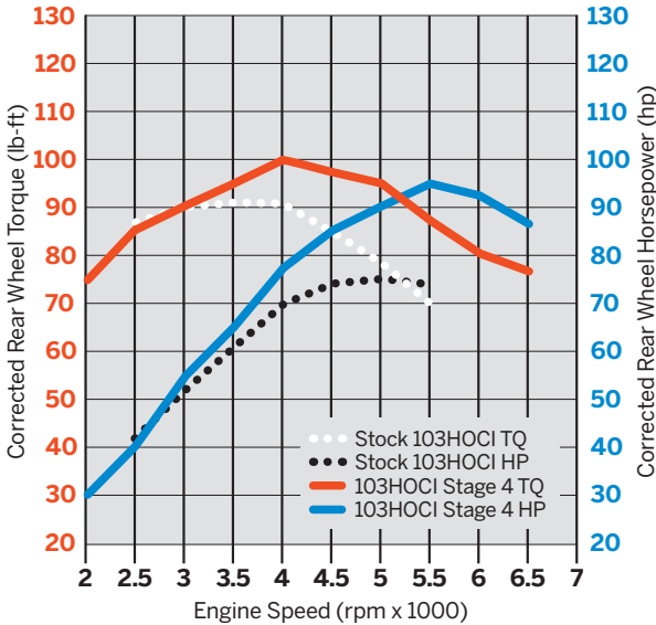
Screamin' Eagle® Street Performance, Twin-Cooled™ Stage 4 Kit – 103 Cubic Inches
