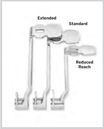
BRAKE LEVER COMPARE – '00-LATER FL SOFTAIL MODELS
