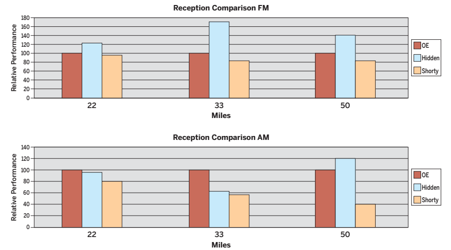
ANTENNA PERFORMANCE COMPARISON – COMPARISON MEASURED ON '06-'13 MODELS WITH ADVANCED AUDIO AM/FM/WB RADIO
