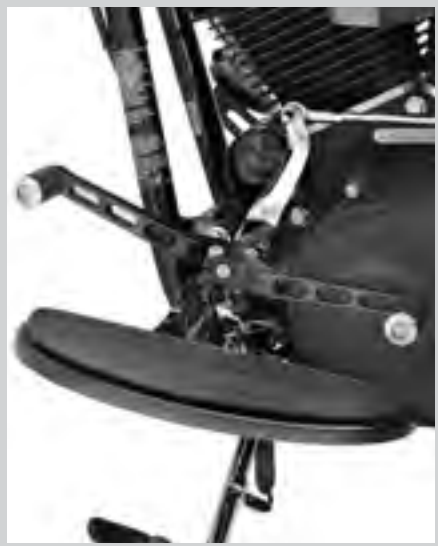
C. BILLET STYLE HEEL/TOE SHIFT LEVER – SATIN BLACK
