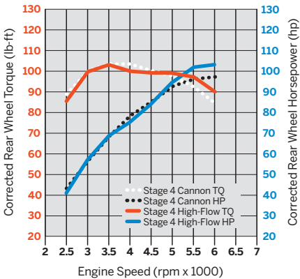
TWIN CAM 103 STAGE 4 HIGH-FLOW VS. OE EXHAUST W/STREET CANNONS
